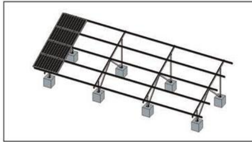
Step 5: Fix panel on rail until finished.
